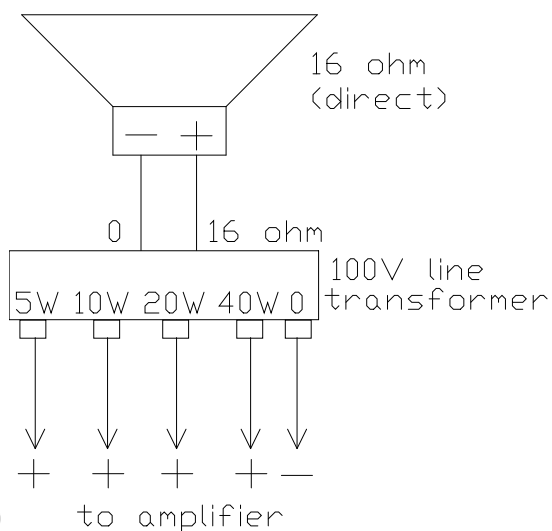
Fig. 2. CS7 wire connection (with transformer TF-100)
