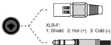
TRS Tip/Ring/Sleeve Combo-XLR jack
